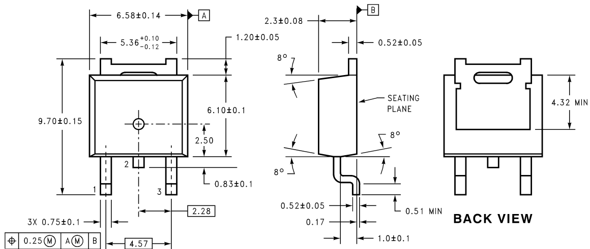
Order Number LM317S NS Package Number TS3B
