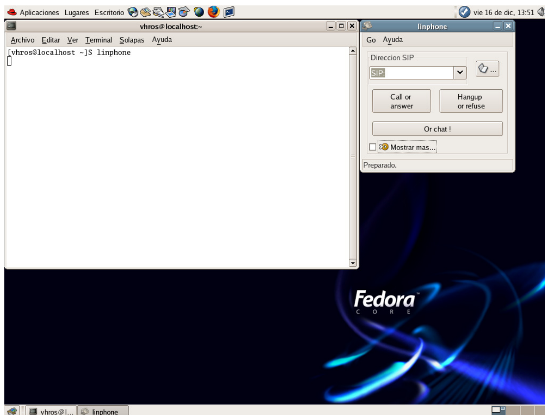
Figura 4.11: Arrancando Linphone.
