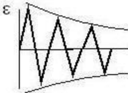
Strain response for cyclic hardening
