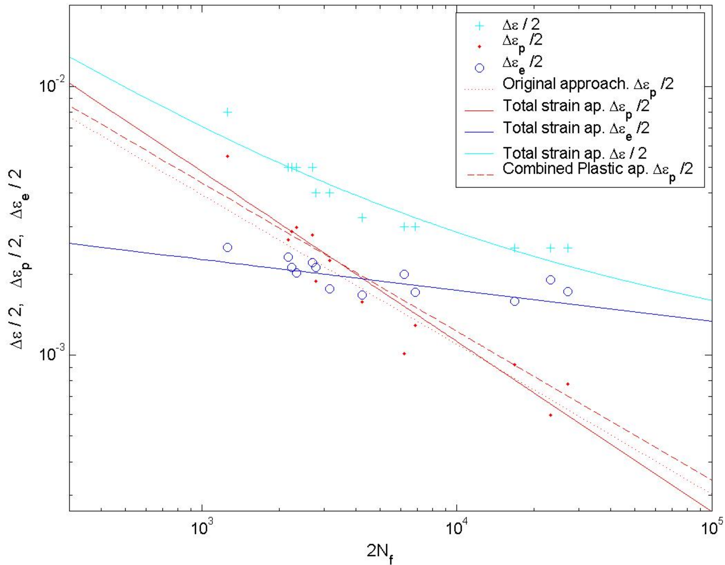
Different approaches to total fatigue life
