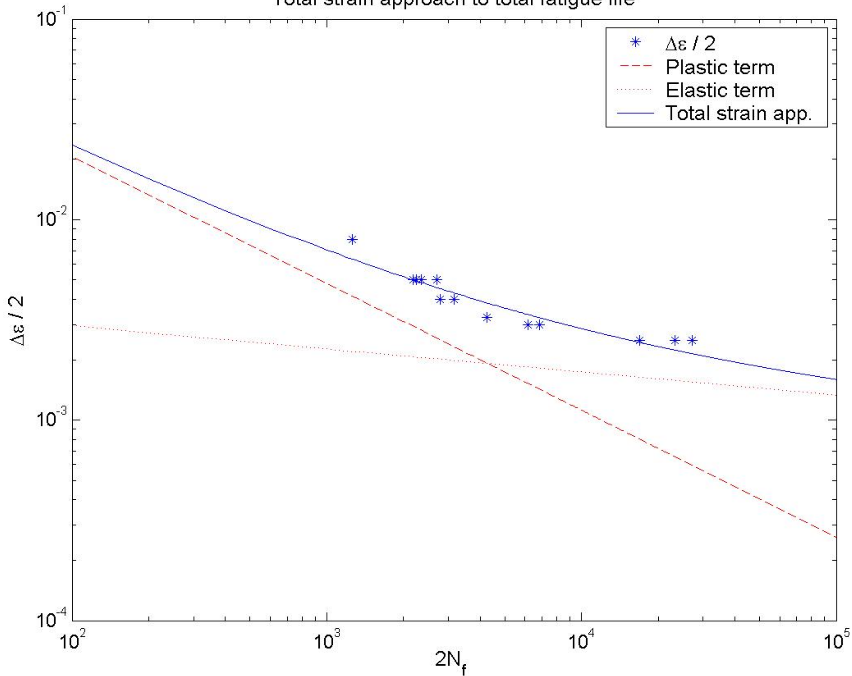
Total strain approach to total fatigue life
