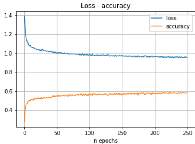
Figura 23. Red neuronal Fully connected . Ensayo 6
