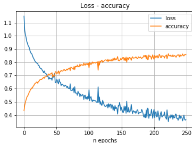
Figura 36. Red neuronal Fully connected . Ensayo 19
