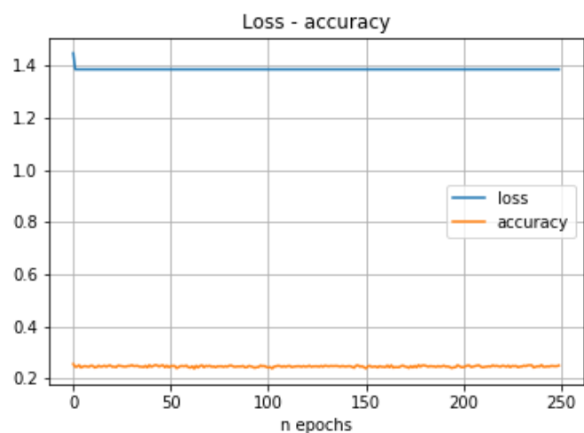
Figura 24. Red neuronal Fully connected . Ensayo 7
