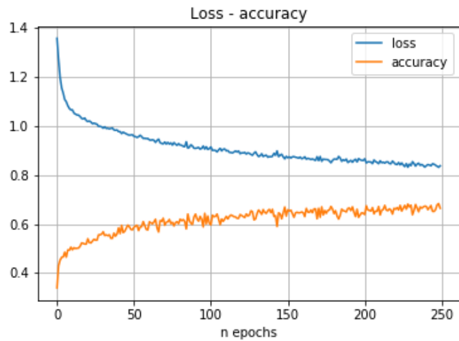
Figura 27. Red neuronal Fully connected . Ensayo 10
