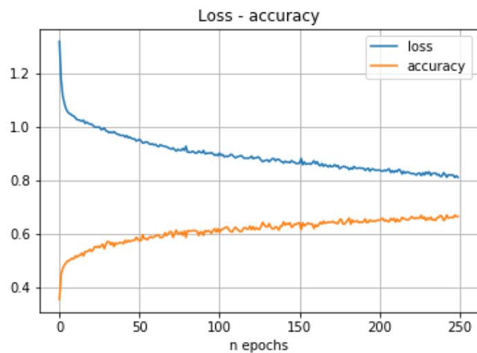
Figura 30. Red neuronal Fully connected . Ensayo 13
