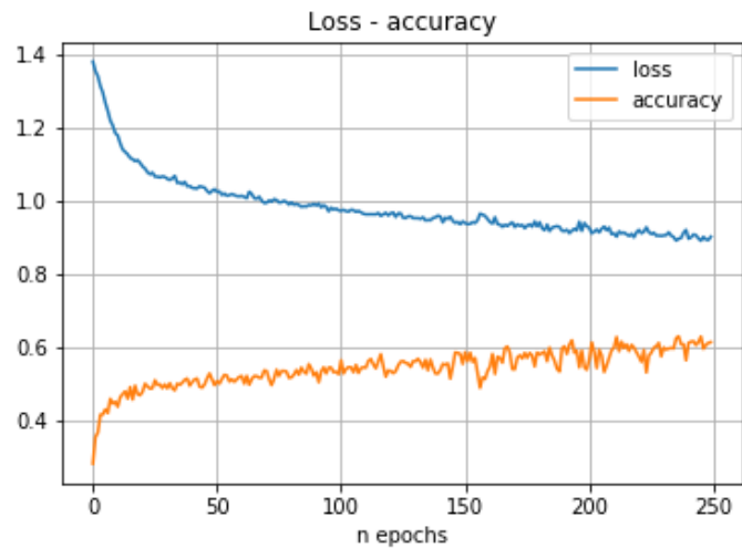
Figura 25. Red neuronal Fully connected . Ensayo 8
