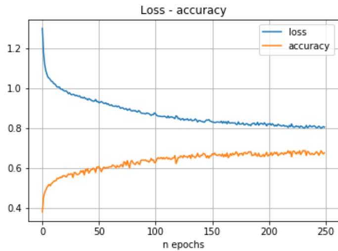
Figura 29. Red neuronal Fully connected . Ensayo 12
