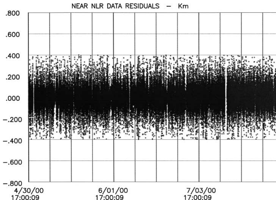
FIG. 3. NEAR spacecraft NLR residuals. The rms error is about 100 m after data points with an error greater than 400 m are rejected.
