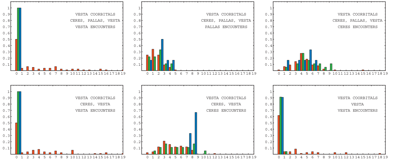
Fig. 12. As Fig. 11 but for Vesta co-orbitals.
