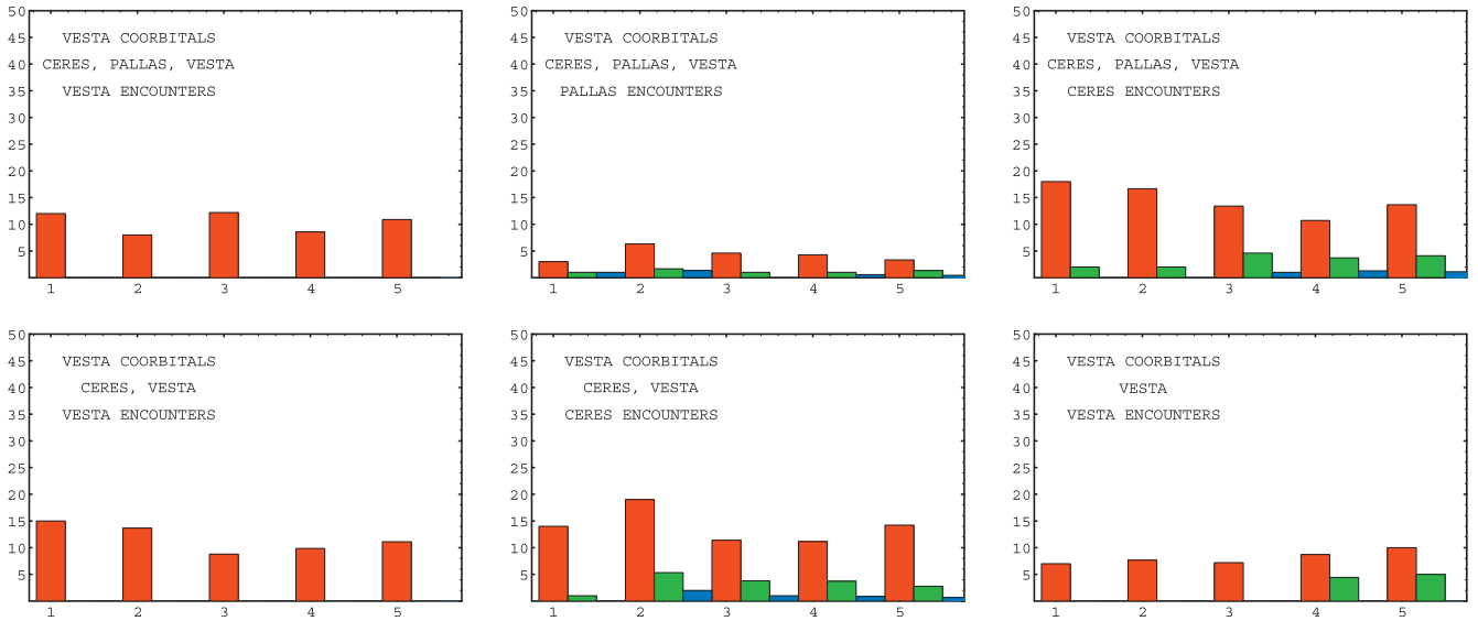
Fig. 14. As Fig. 13 but for Vesta co-orbitals.
