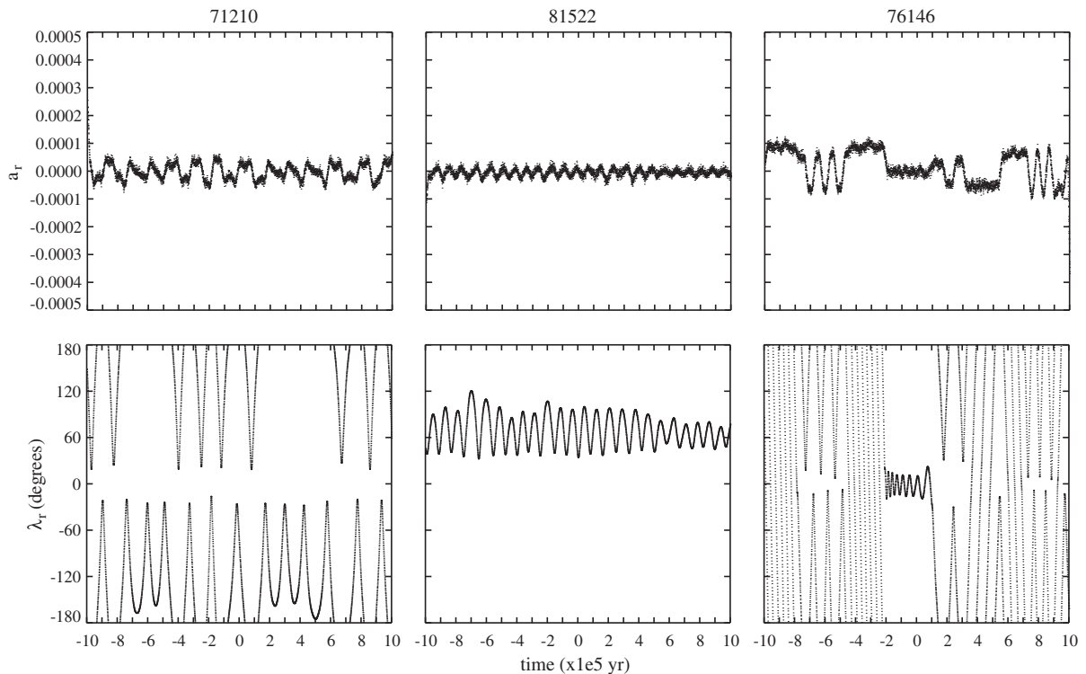
Fig. 2. Examples of dynamical evolution of specific asteroids coorbiting with Ceres as determined by our numerical integrations over 2 \times 10^6 yr. The upper row shows the evolution of the relative semimajor axis a_r while the bottom row that of the relative longitude \lambda_r .
