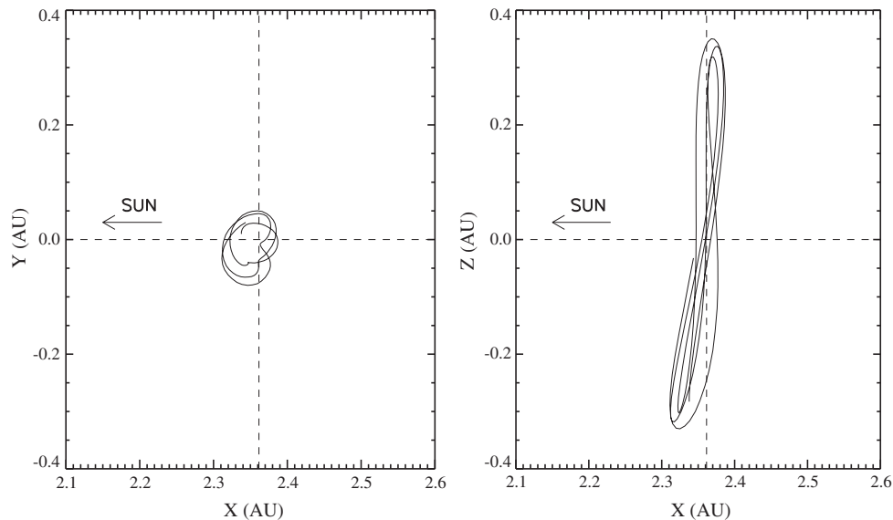
Fig. 19. Motion of 139168 with respect to Vesta in cartesian ecliptic coordinates during an episode of QS capture at t \simeq -3 \times 10^5 yr indicated in Fig. 18. The dashed lines mark the location x = a_{p, \text{Vesta}} \simeq 2.3615 AU, y = z = 0 . Note the large amplitude of the vertical motion (right panel) compared to the planar projection (left panel).
