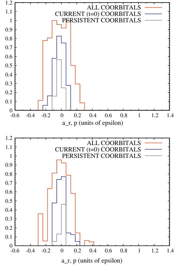
Fig. 6. Histograms of the statistical distribution of different types of Ceres (top) and Vesta (bottom) co-orbital asteroids divided over the total number of asteroids in each bin. The x-axis is in the same units as Fig. 5.
