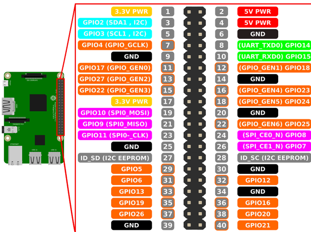
Figura 4:8 GPIO Raspberry Pi 3 Model B.
