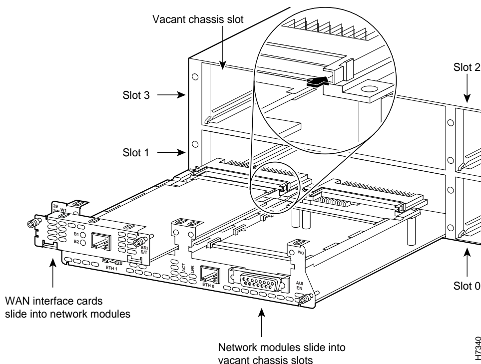
Figure 18-11: Relationship Between Cisco 3600 Series Hardware Devices
