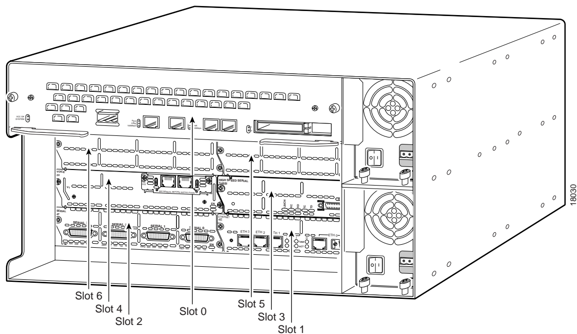
Figure 18-8: Cisco 3660 Router Rear View
