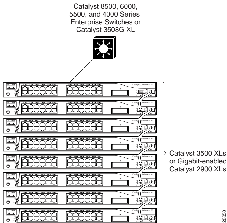
Figure 21-9: Creating an Independent Stack Bus
