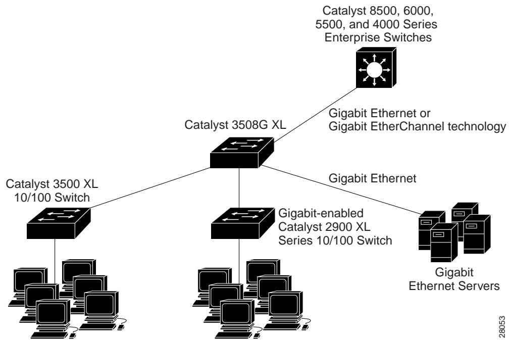
Figure 21-12: Enterprise Workgroup Aggregation
