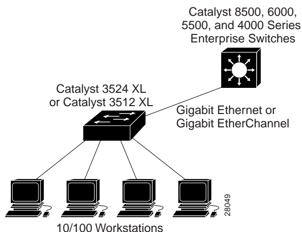
Figure 21-8: Catalyst 3512 XL or Catalyst 3524 XL for Desktop Connectivity
