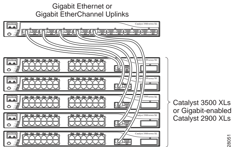
Figure 21-10: Point-to-point stacking
