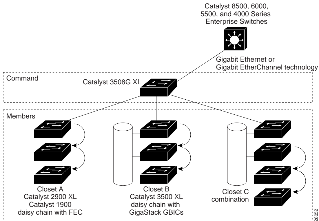
Figure 21-11: Cisco Switch Clustering
