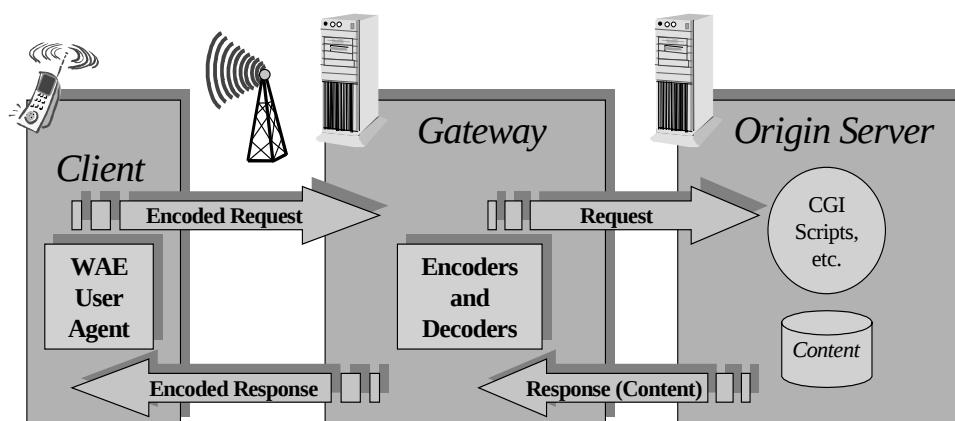
Figure 2. WAP Programming Model
