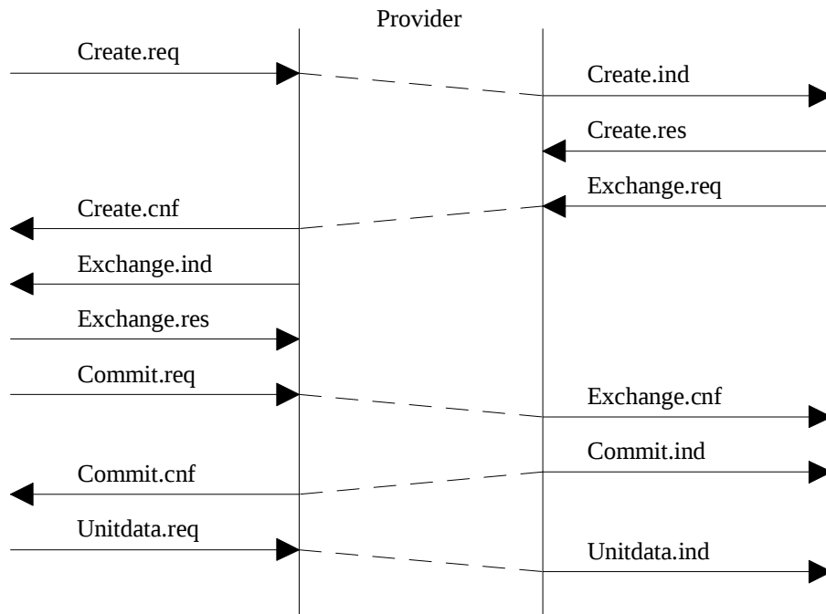
Figure 3: Full Handshake
