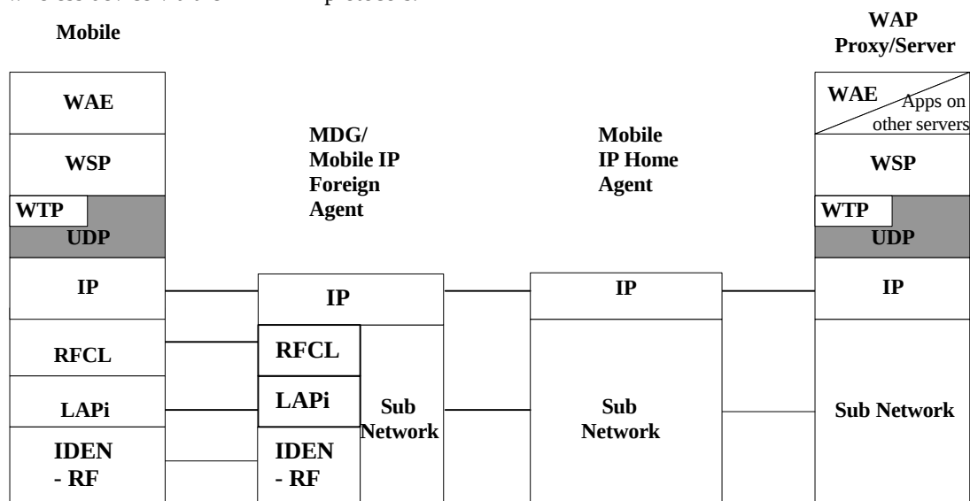
Figure 5.22: WTP over iDEN Packet Data
