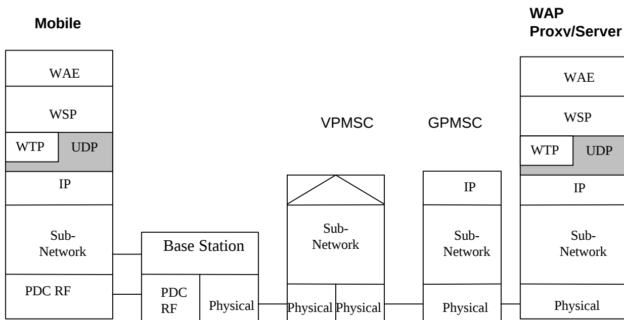
Figure 5.20: WDP over PDC Packet Data Channel
