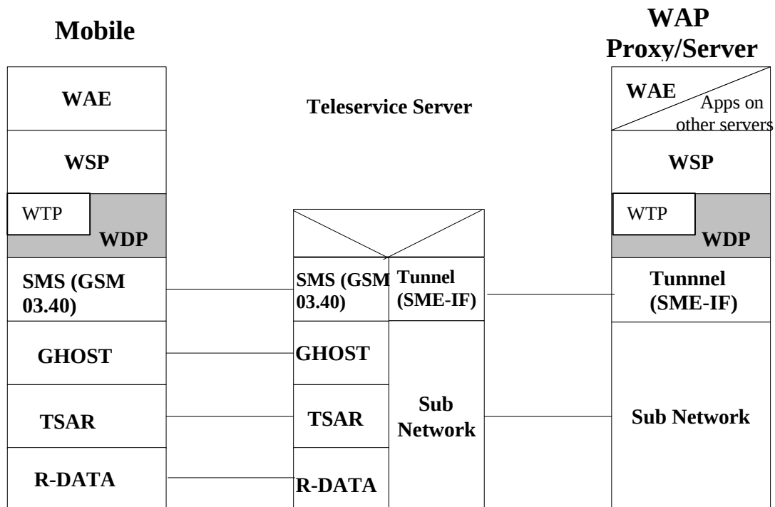
Figure 5.10 illustrates the protocol profile for the WDP layer when operating over the ANSI-136 GHOST and R-DATA bearer service. Note that Teleservice Segmentation and Reassembly (TSAR) is optional.
