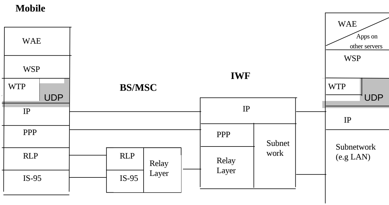
Figure 5.16: WDP over CDMA Packet Data Channel
