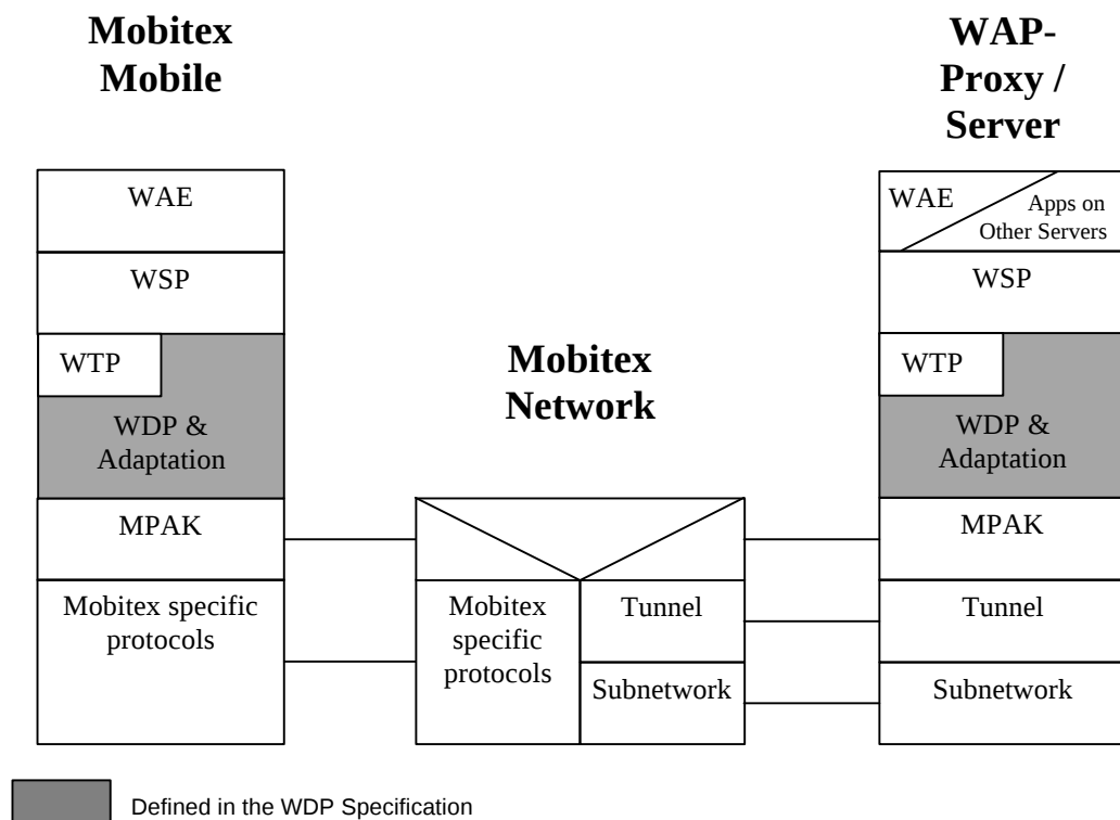
Figure 5.32: WDP over Mobitex.
