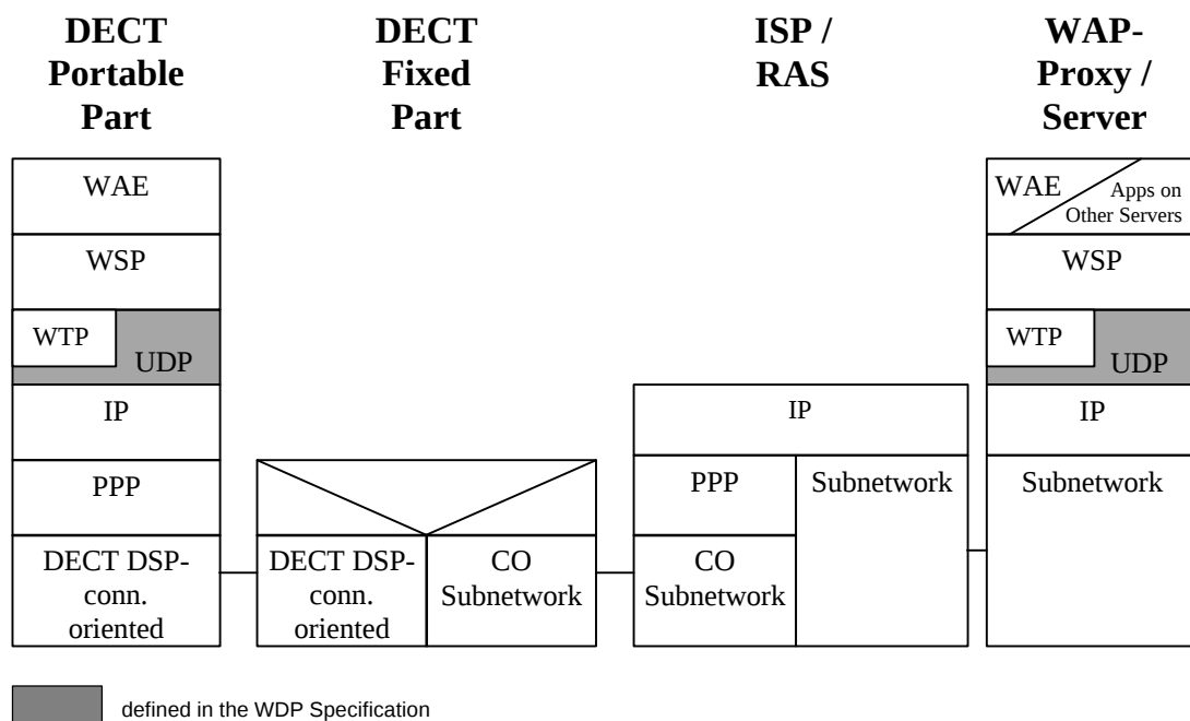
Figure 5.30: WDP over DECT connection oriented services.
