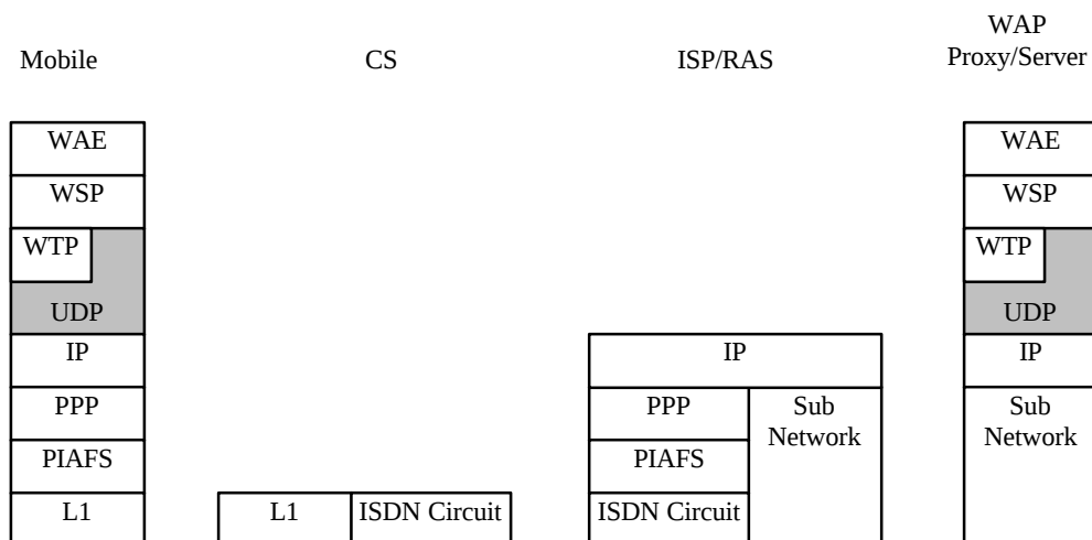
Figure 5.25: WDP over PHS Circuit-Switched Data Channel
