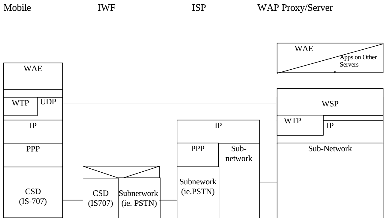
Figure 5.15:WDP over CDMA Circuit-Switched Data Channel
