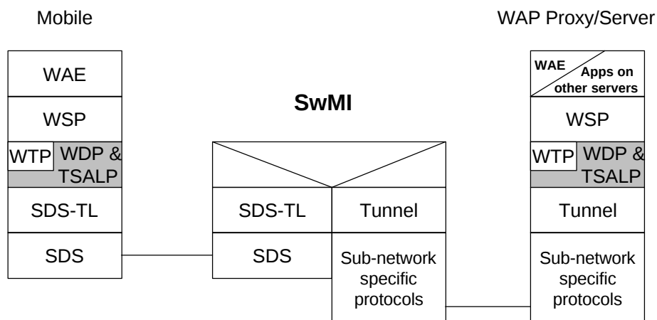
Figure 5.27 WDP over TETRA SDS; WAP Proxy/Server is external to SwMI
