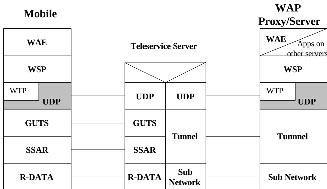
Figure 5.9: WDP over ANSI-136 R-DATA using GUTS
