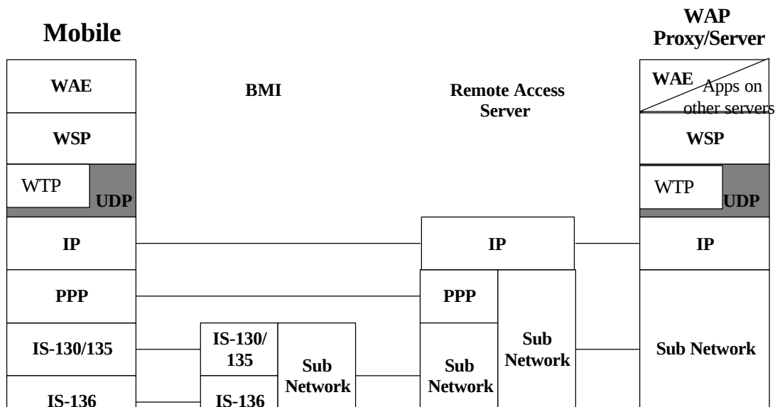
Figure 5.11: WDP over ANSI-136 Circuit-Switched Data
