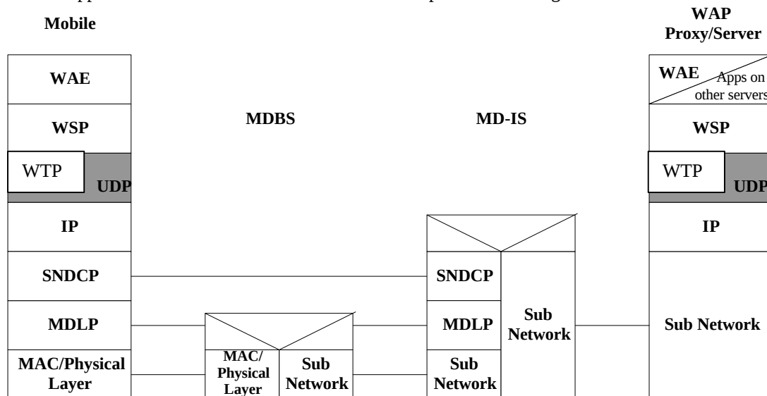
Figure 5.13: WDP over CDPD
