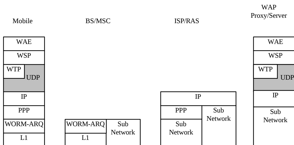
Figure 5.19: WDP over PDC Circuit-Switched Data Channel
