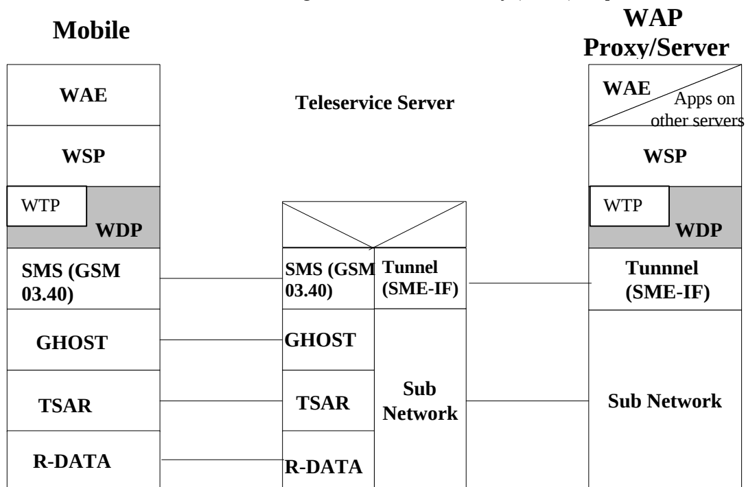
Figure 5.10 illustrates the protocol profile for the WDP layer when operating over the ANSI-136 GHOST and R-DATA bearer service. Note that Teleservice Segmentation and Reassembly (TSAR) is optional.
