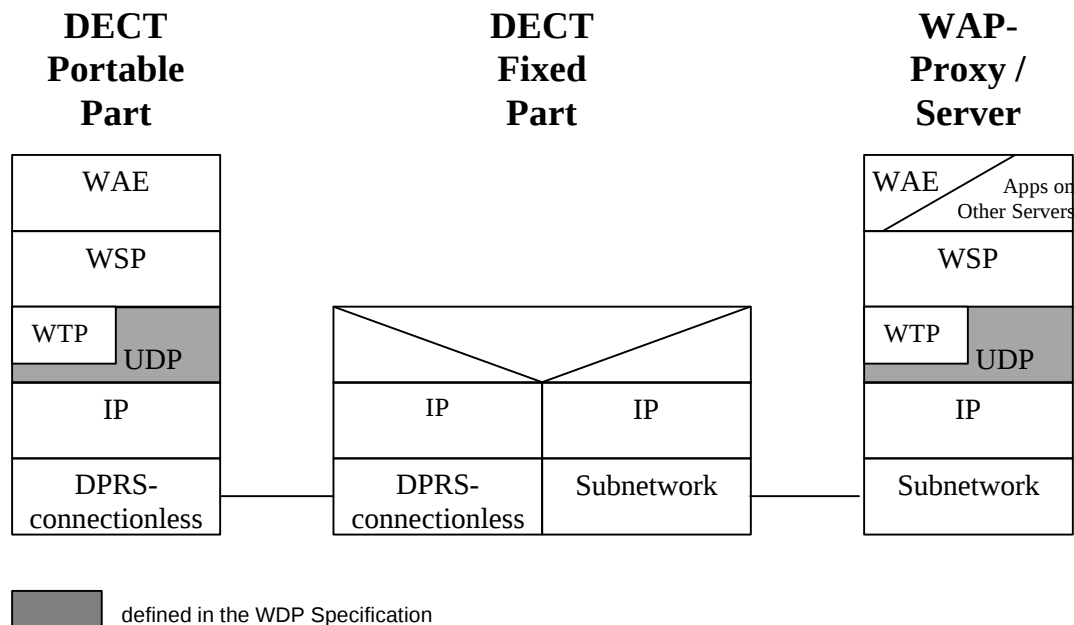
Figure 5.31: WDP over DECT packet switched services.
