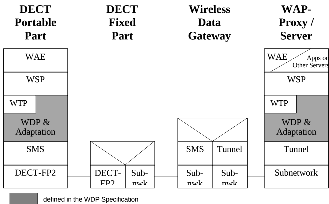
Figure 5.29: WDP over DECT short message service.
