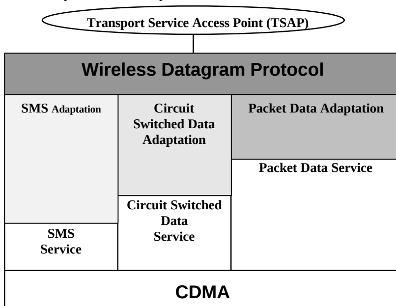
Figure 5.14: WDP over CDMA Bearer Services
