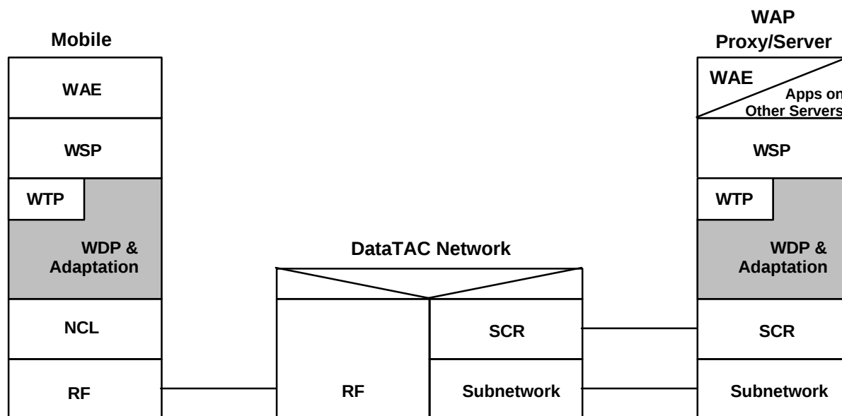
Figure 5.26: DataTAC Profile
