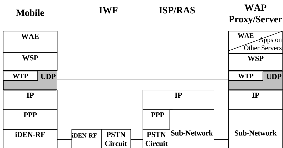
Figure 5.21: WDP over iDEN Circuit-Switched Data Channel
