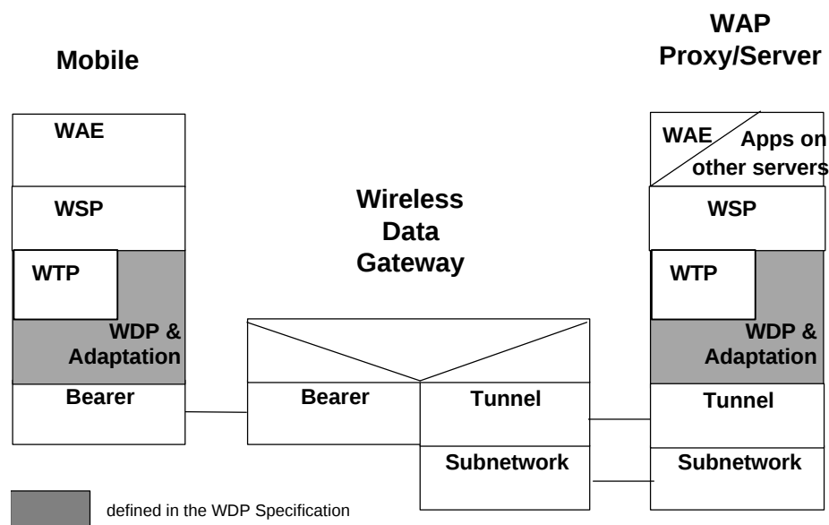
Figure 5.3 General WDP Architecture
