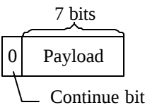
Figure 27. Variable Length Integer Octet
