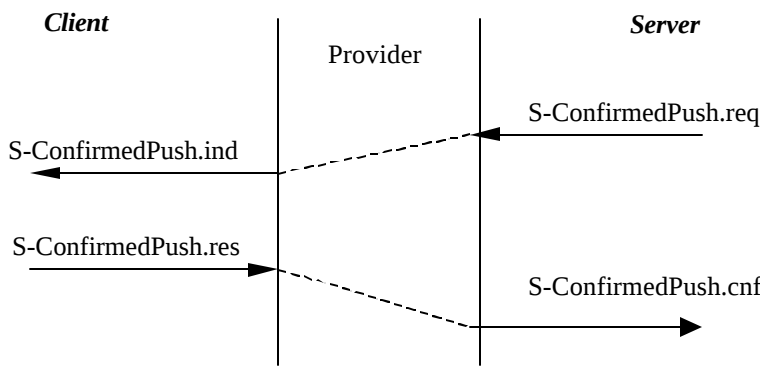
Figure 15: Confirmed Data Push
