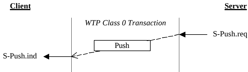
Figure 25. Push Invocation
