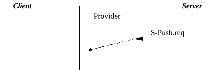
Figure 14: Failed Non-confirmed Data Push
