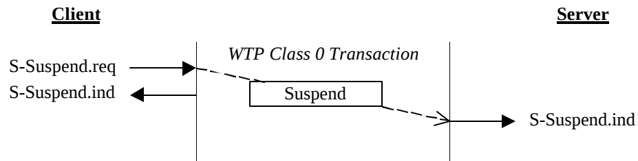
Figure 21. Session Suspend
