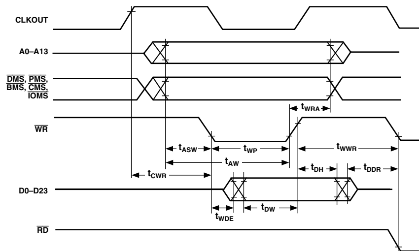
Figure 15. Memory Write
