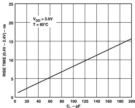
Figure 24. Typical Output Rise Time vs. Load Capacitance, C_L (at Maximum Ambient Operating Temperature)
