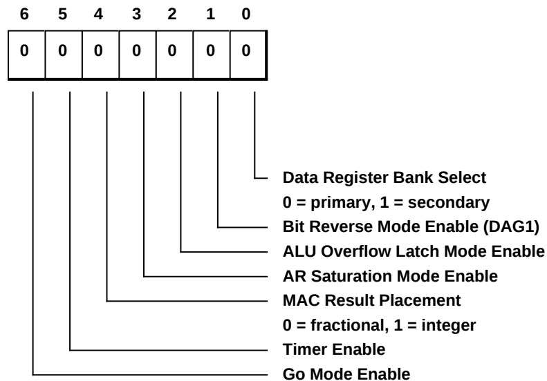
Figure 3.6 MSTAT Register
