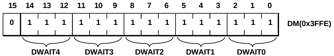
Figure 10.14 Data Memory Waitstate Control Register (ADSP-2101, ADSP-2111, ADSP-2105, ADSP-2115, ADSP-2161/62/63/64)
