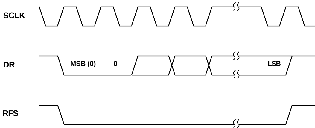
Figure 13.7 SPORT To AD7872 ADC Timing
