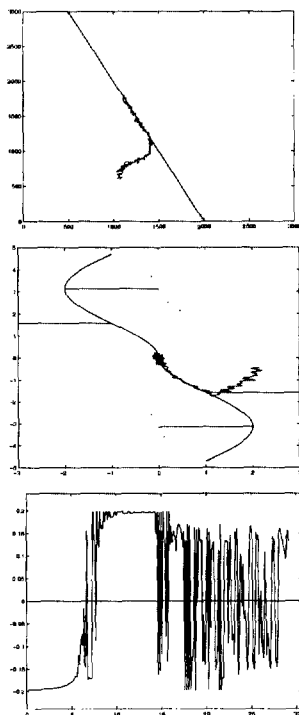
Figure 5: Experiment 1: (Chattering control) From top down: reference route and vehicle position during execution of the control law; the same positional data in the reduced state space; control input vs. time.
