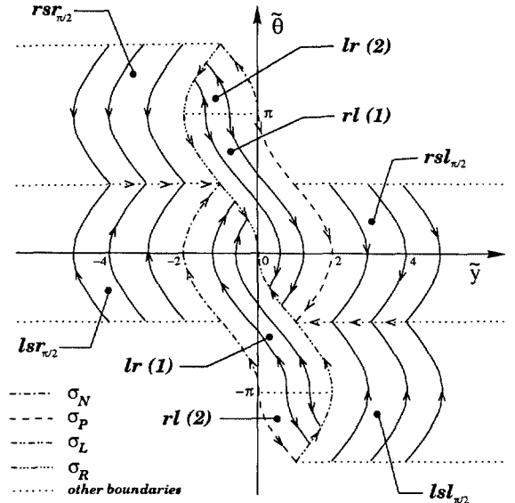
Figure 3: Optimal synthesis in the (\tilde{y}, \tilde{\theta}) -plane.
