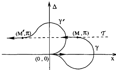
Figure 2: Isometric paths r_{(\pi R+a)}l_a and l_ar_{(\pi R+a)}
