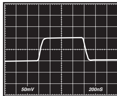
TPC 27. Small-Signal Transient Response
