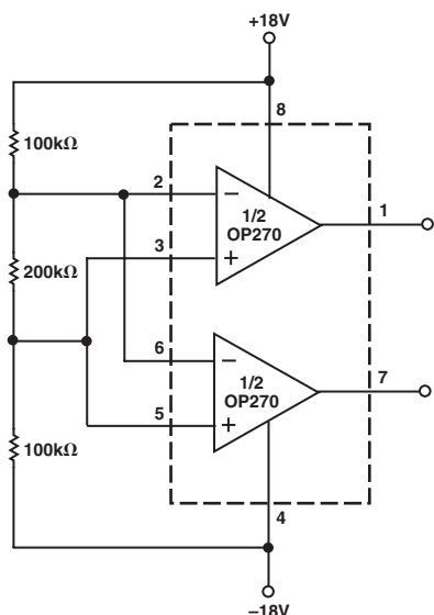
Figure 2. Burn-In Circuit
