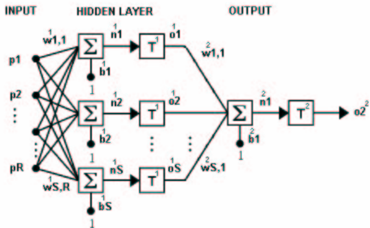
Multiple layers of neurons
