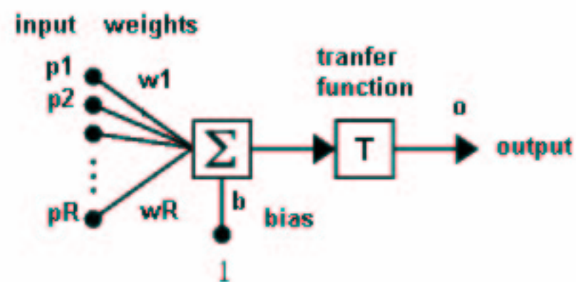
Neuron with input vector
