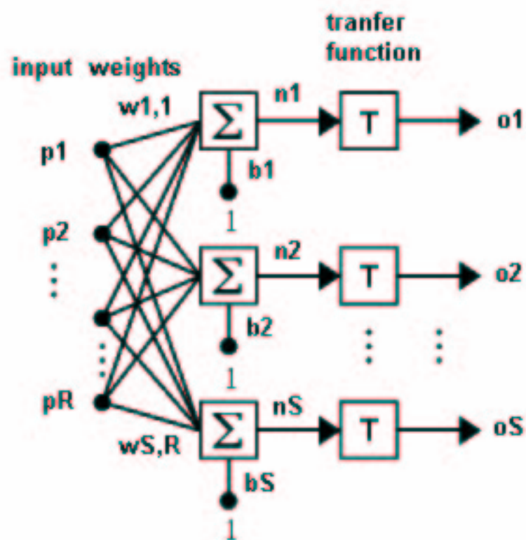
Layer of S neurons
