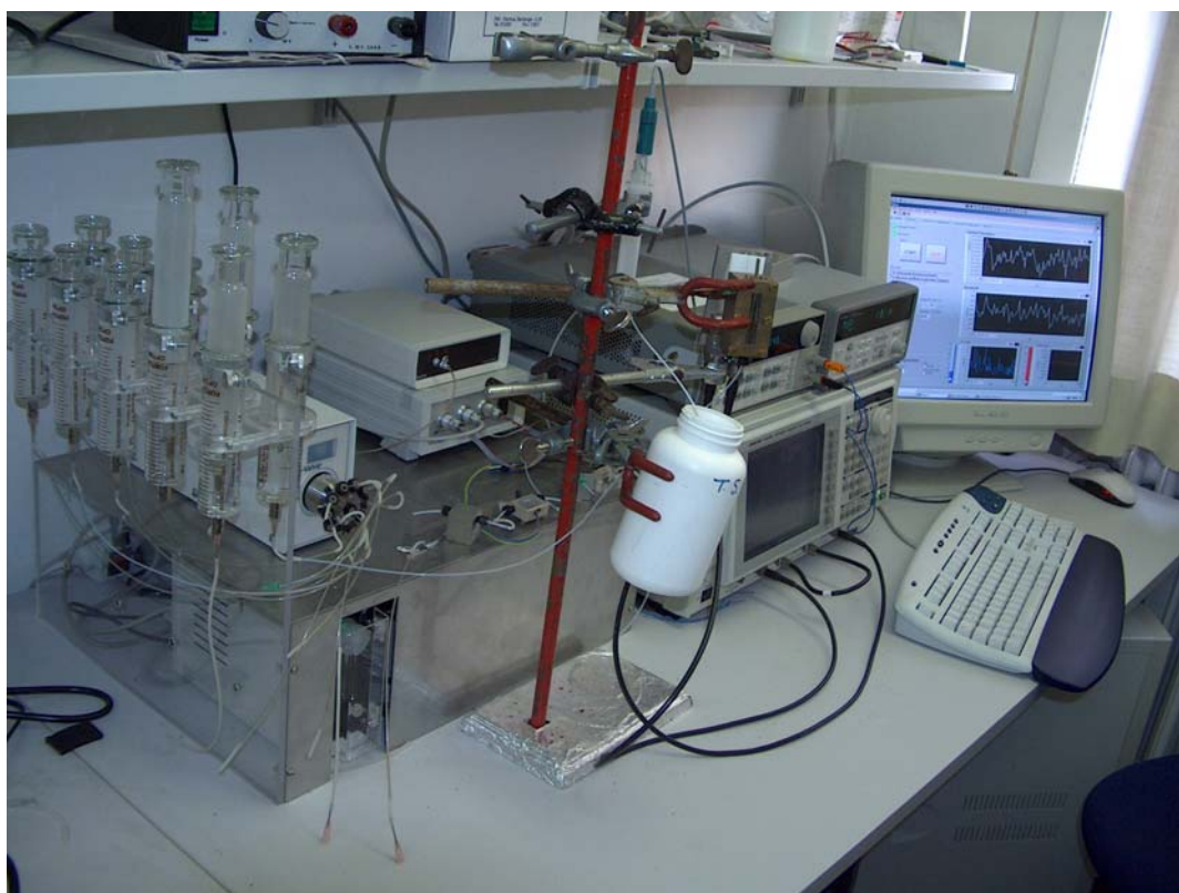
Testbench: Complete Set
