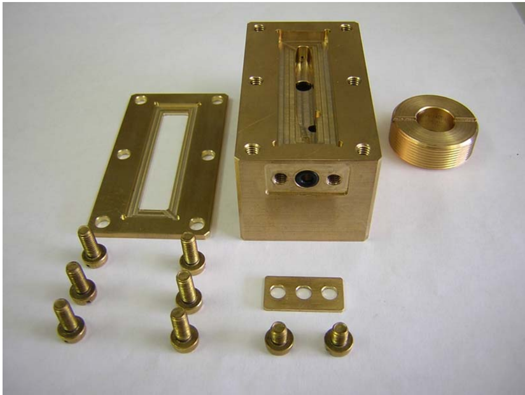
Measurement cell: Exploded View
