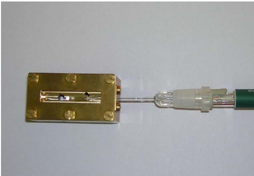
Measurement cell: pH sensor Insertion
