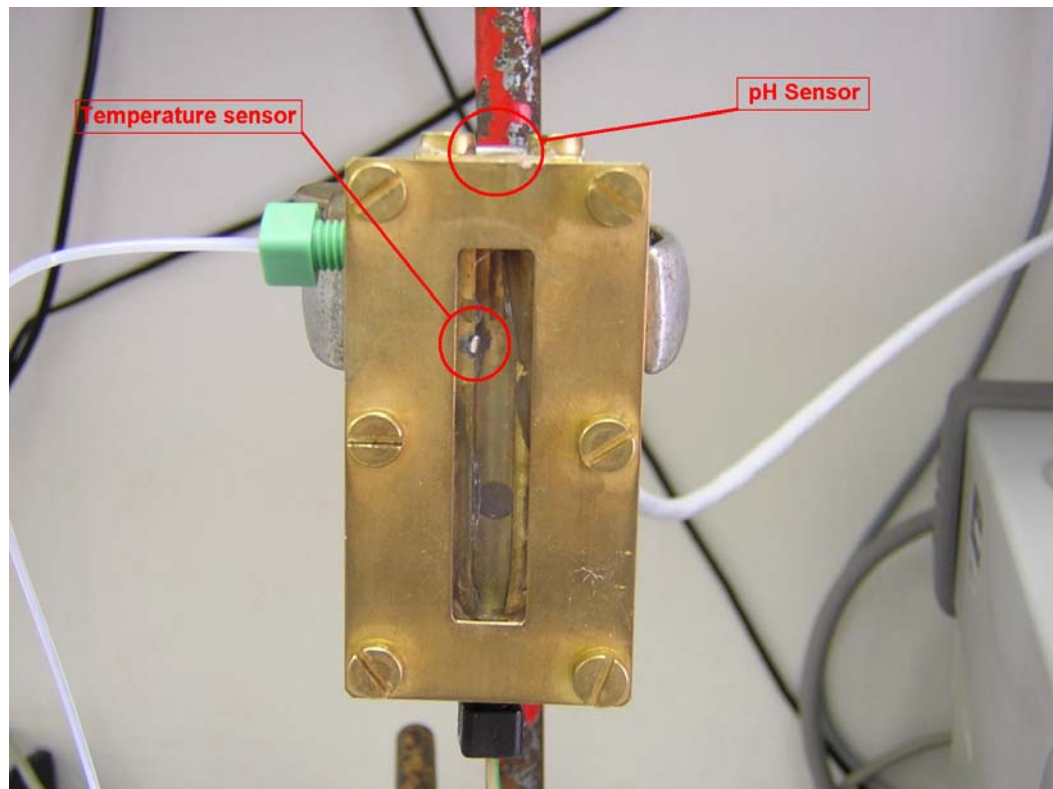
Measurement cell: Detailed view
