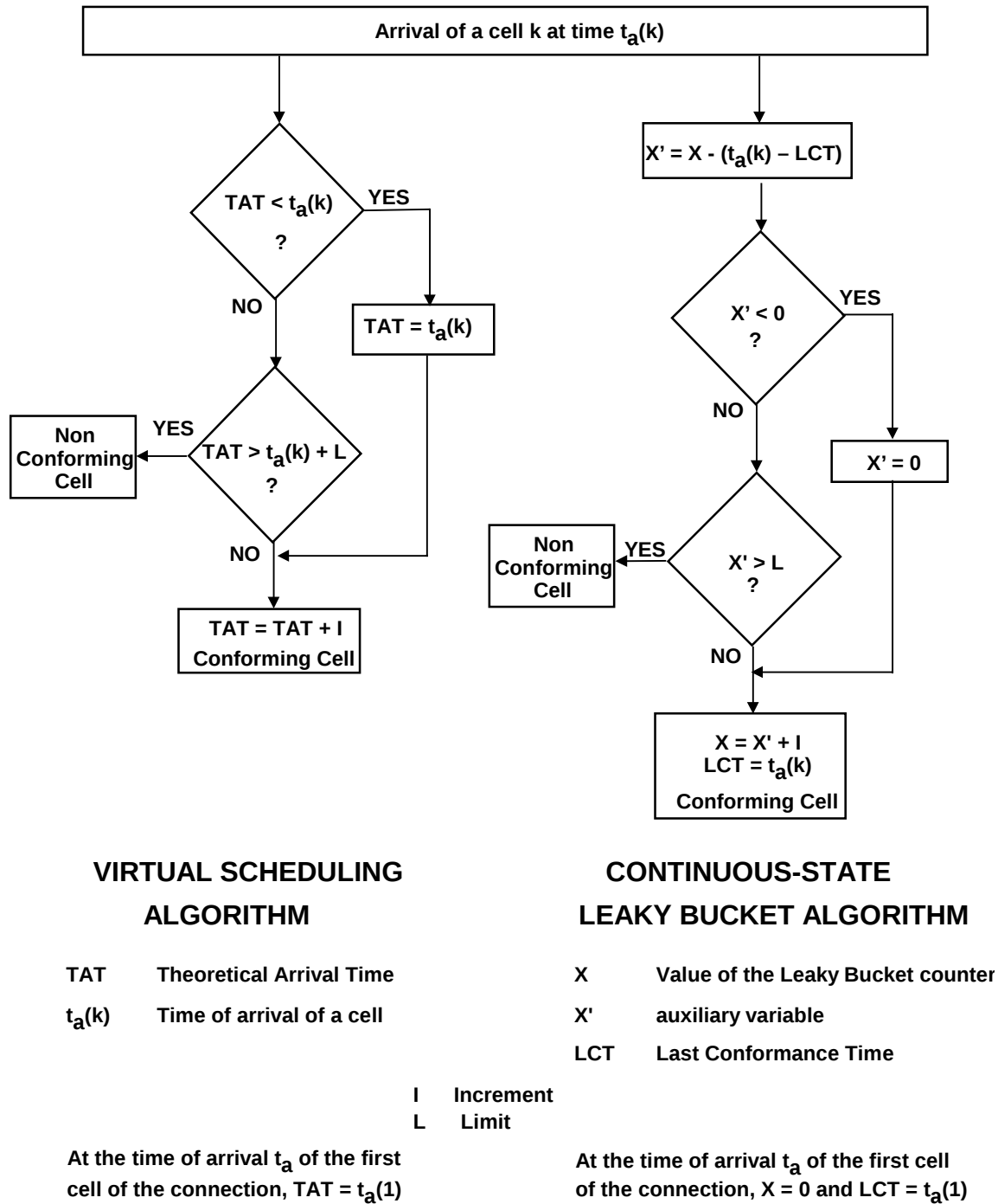
Figure B-1: Equivalent versions of the Generic Cell Rate Algorithm (same as Figure 4-1)
