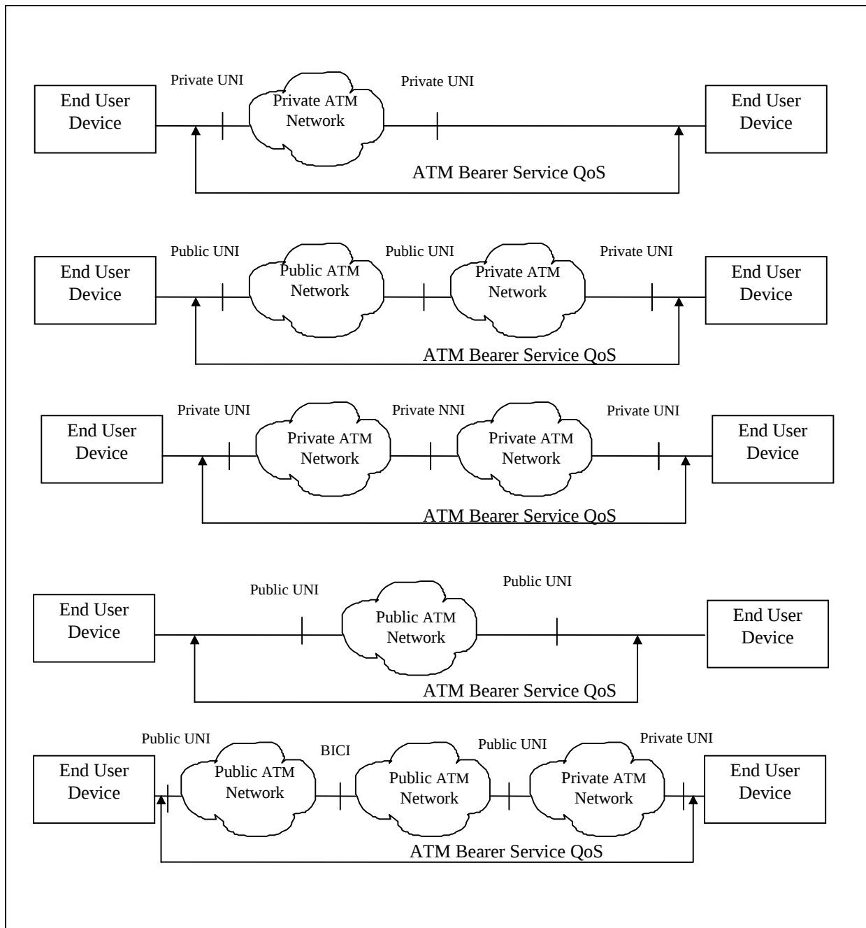
Figure 3-1: ATM QoS Reference Configurations
