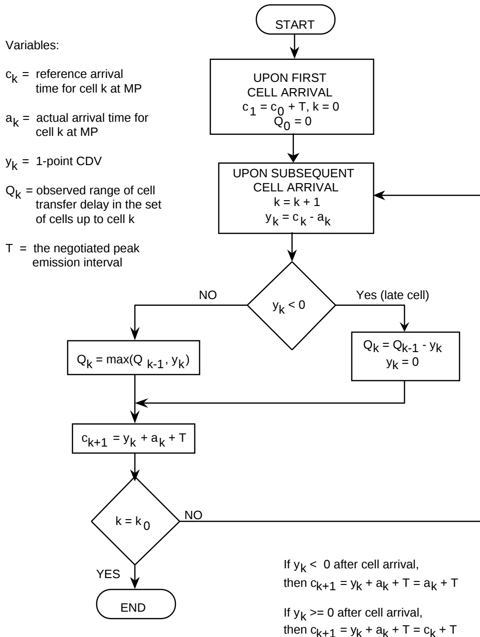
Figure VII-1: Estimation of the range of two-point CDV from one-point CDV for connections providing CBR service
