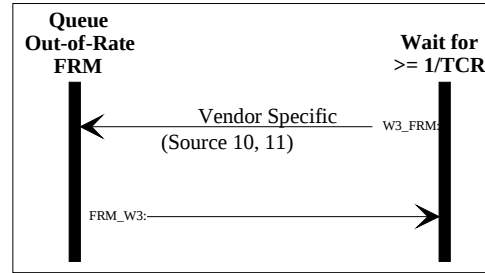
Source Out-of-Rate Forward RM Generation (State Machine #3)
