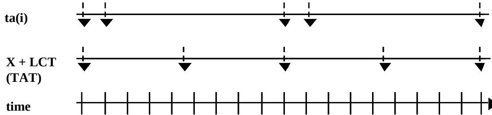
Figure B-4: Possible Cell Arrival at the Public UNI ( \tau = 3.5\delta )
