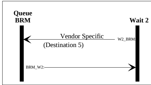
Destination Generated Backward RM (BN=1) (State Machine #2)
