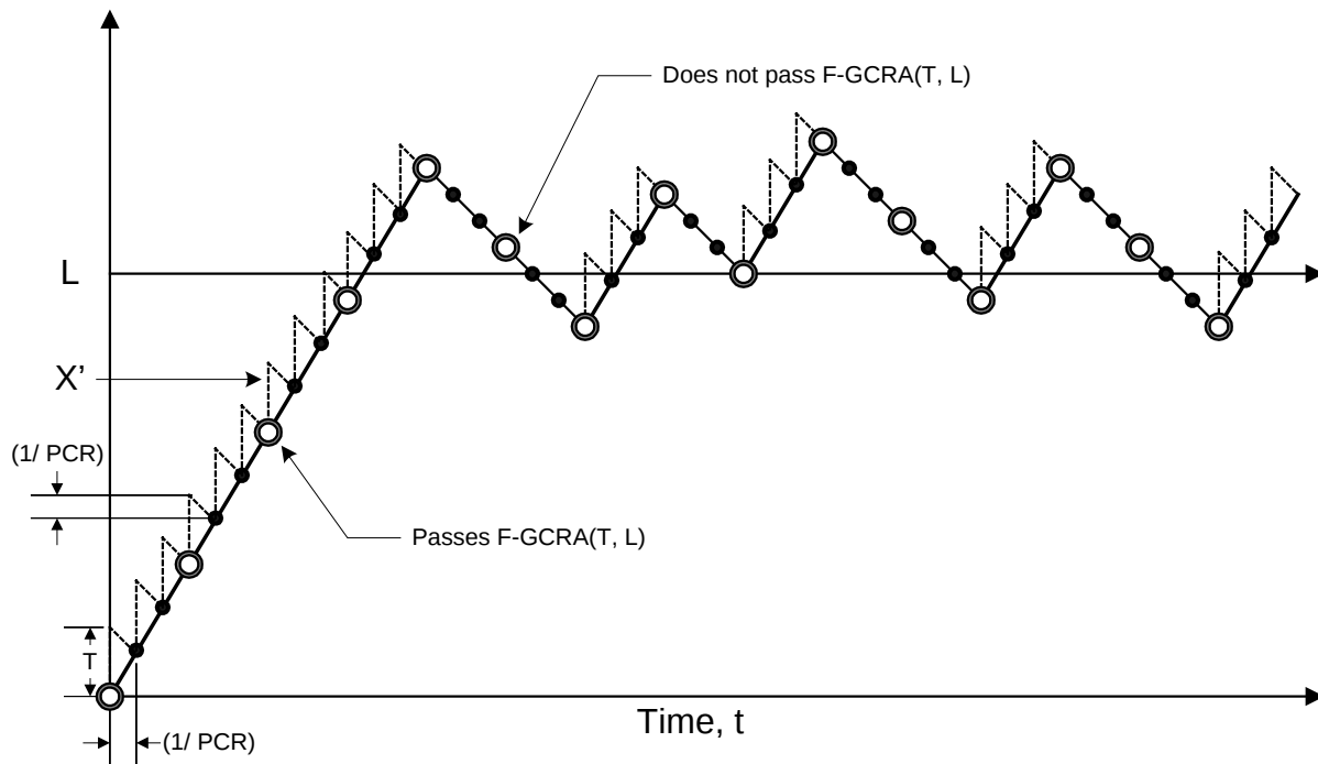
Figure VI-2 F-GCRA state variable as a function of time.
