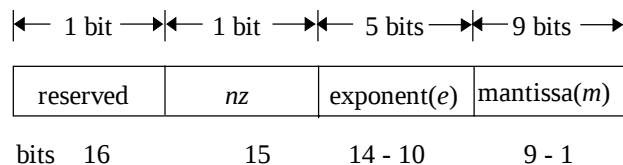
Figure 5-4: Rate format used in RM-cells
