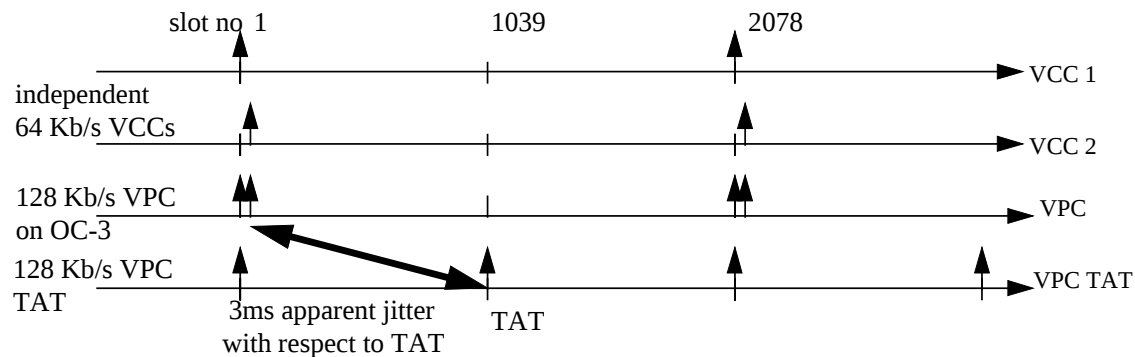
Figure V-1 Apparent VPC jitter produced by independent CBR VCCs
