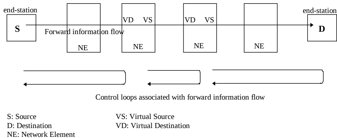
Figure 5-5: Example of a segmented ABR virtual connection
