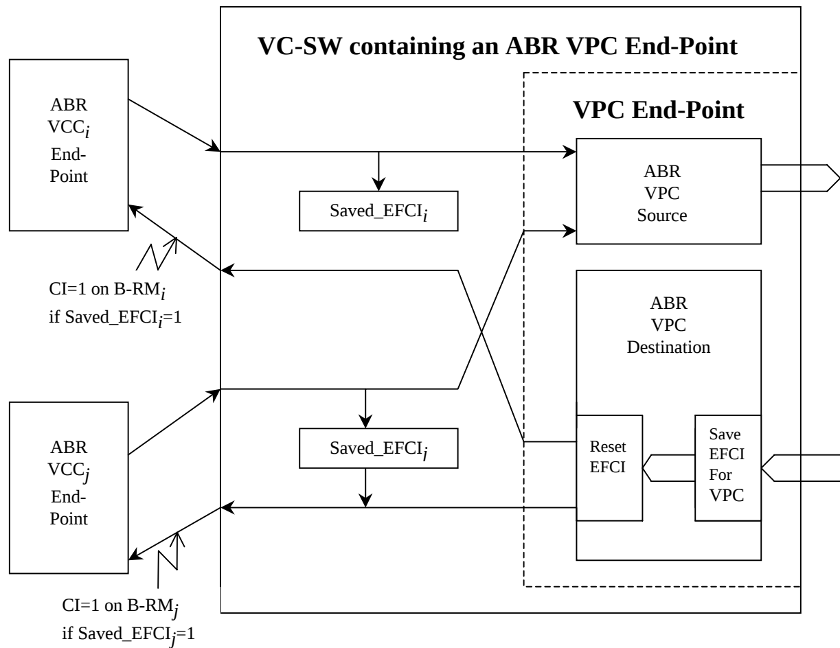
Figure 5-7: VC-Sw containing ABR VPC End-Point Satisfying Requirements (a) and (b)
