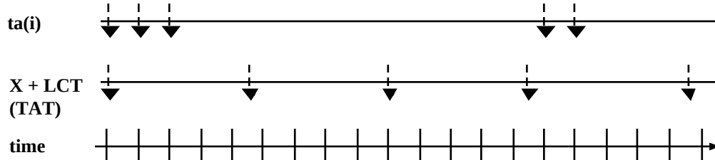
Figure B-5: Possible Cell Arrival at the Public UNI ( \tau = 7\delta )
