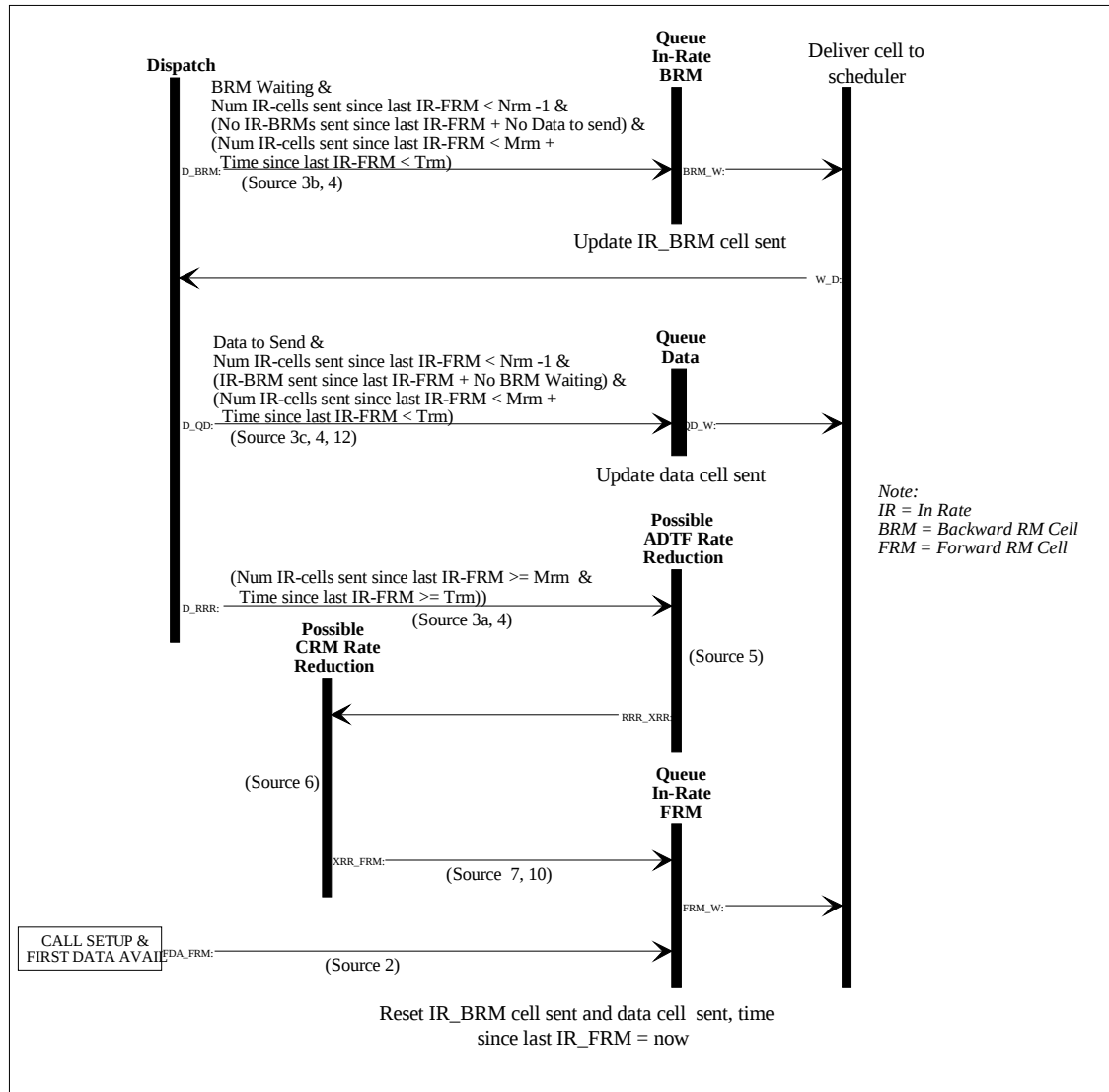
Generation of In-Rate Cells (Data, Forward and Backward RM- (State Machine #1)
