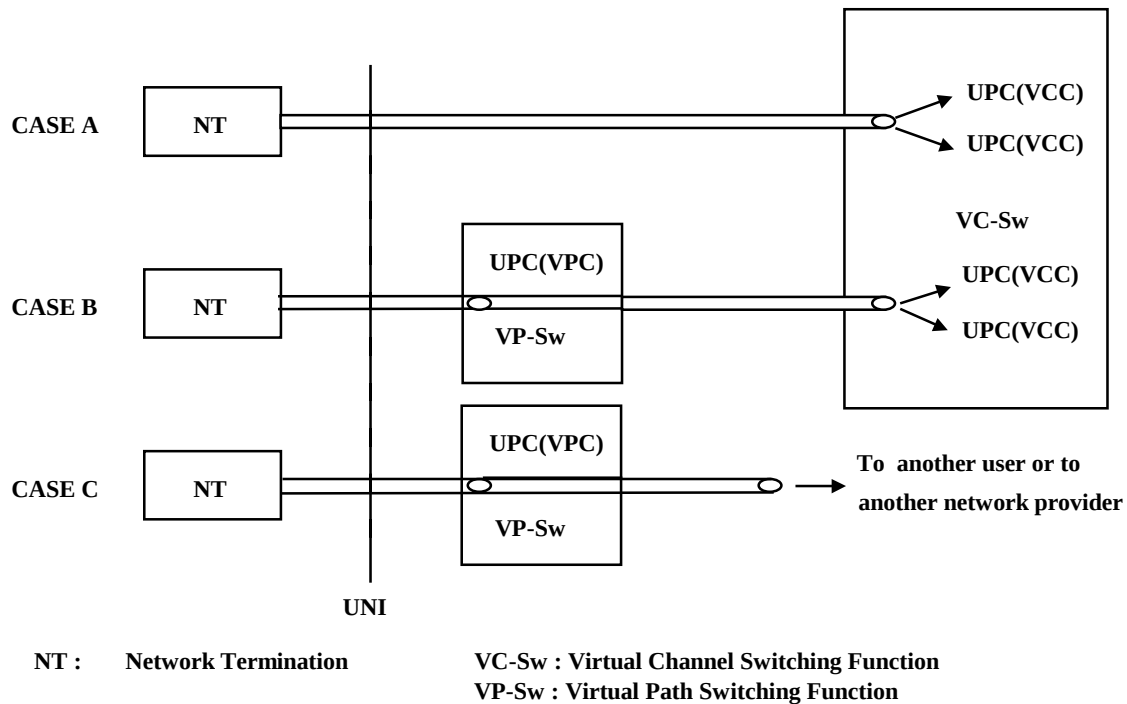
Figure 5-1: Location of the UPC Functions
