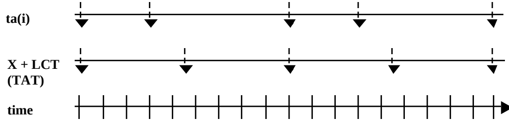
Figure B-3: Possible Cell Arrival at the Public UNI ( \tau = 1.5\delta )
