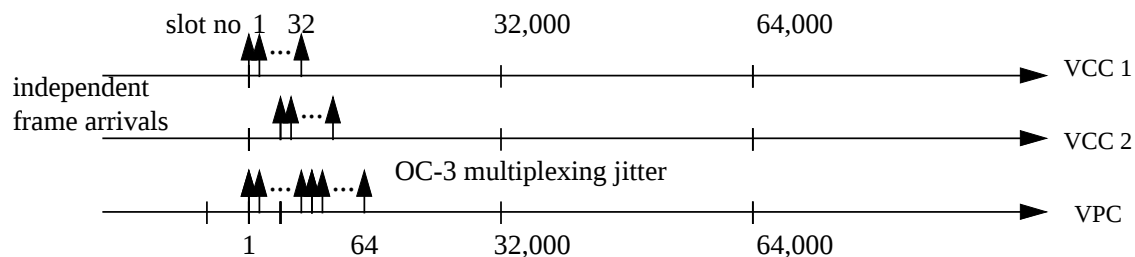
Figure V-2 Apparent MBS escalation produced by independent VBR VCCs
