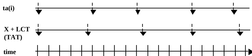
Figure B-2: Ideal Cell Arrival at the Public UNI ( \tau = 0.5\delta )
