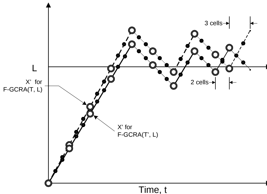
Figure VI-3 State variables of distinct F-GCRA instances.
