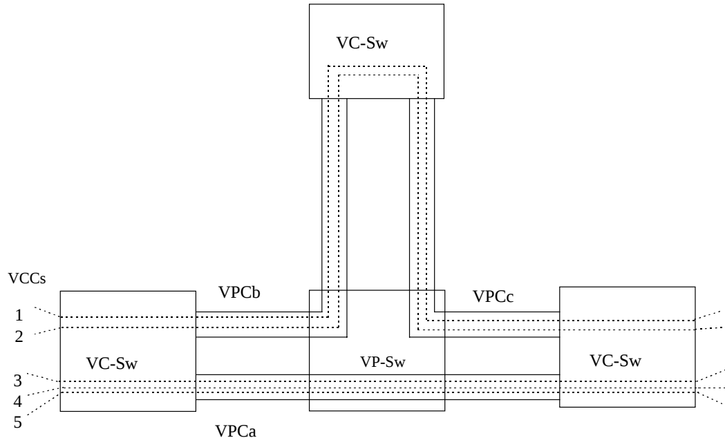
Figure 5-2: Mapping cell loss ratios for VCC and VPC
