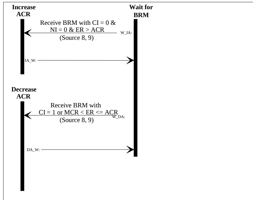
Backward RM Reception (State Machine #4)
