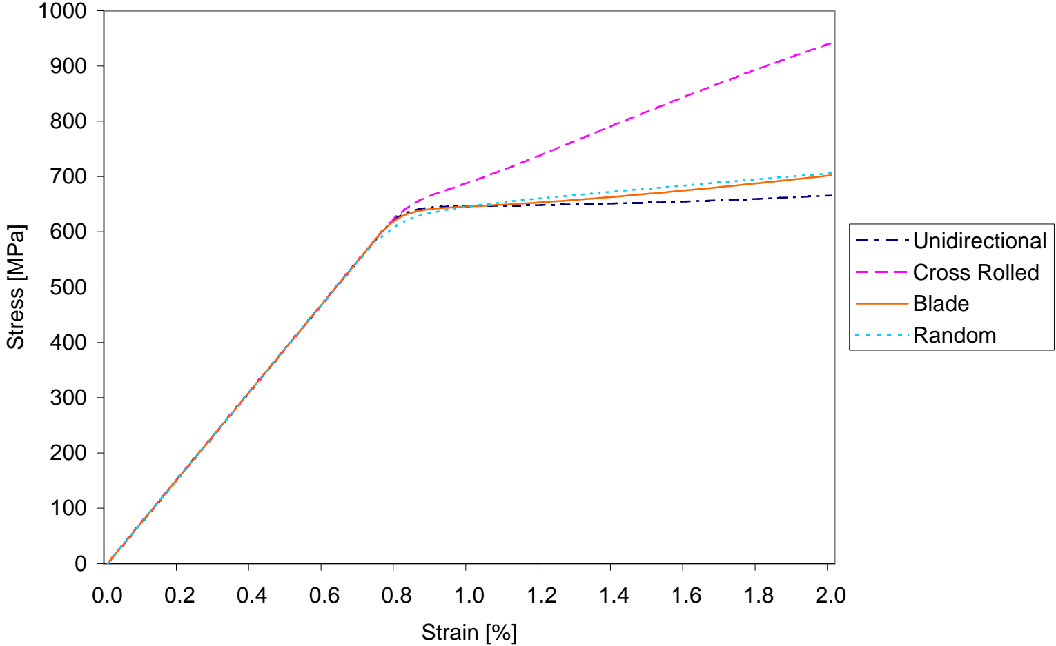
Stress-Strain Curves
